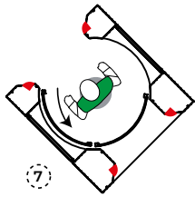
Exit door opens after 2nd level access control approval (**)
